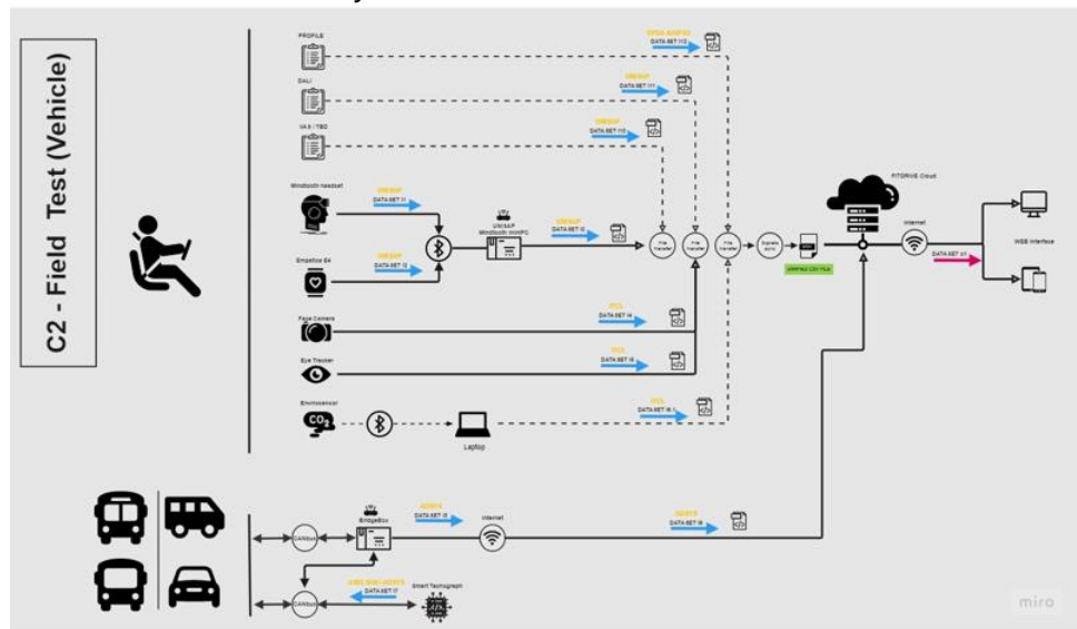
Figure 7: Scheme of the cloud-based data transmission.
